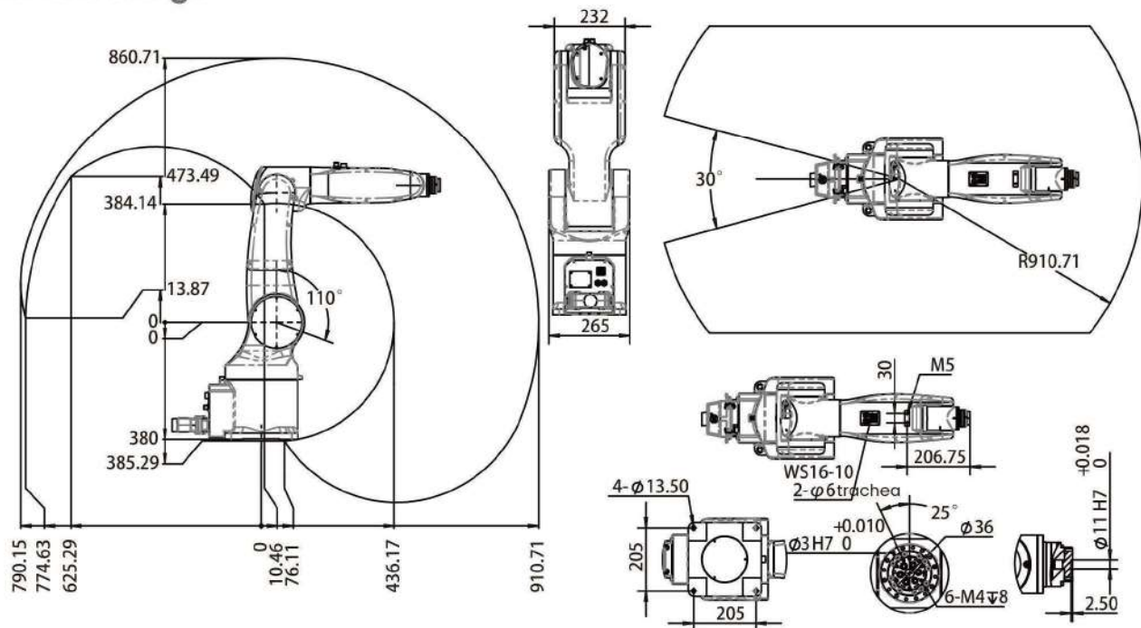
Base installation drawing
